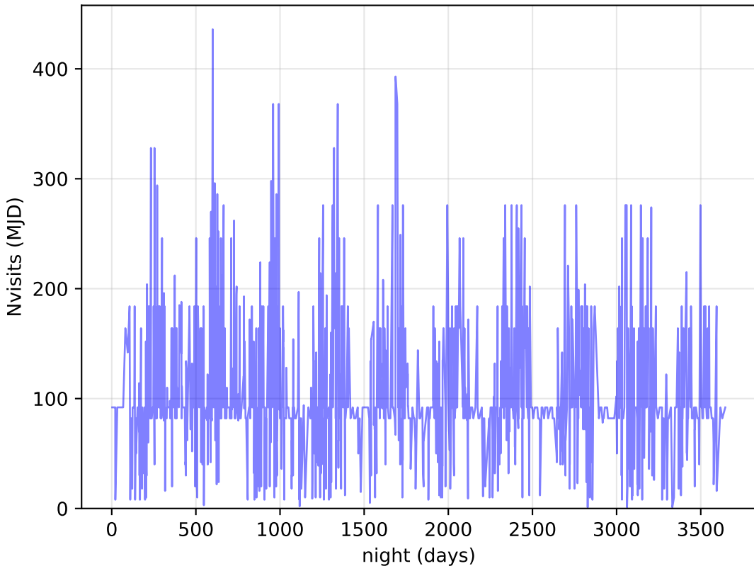
internal_u_expt45_nscale0.9v3.4_10yrs DDF: Nvisits
