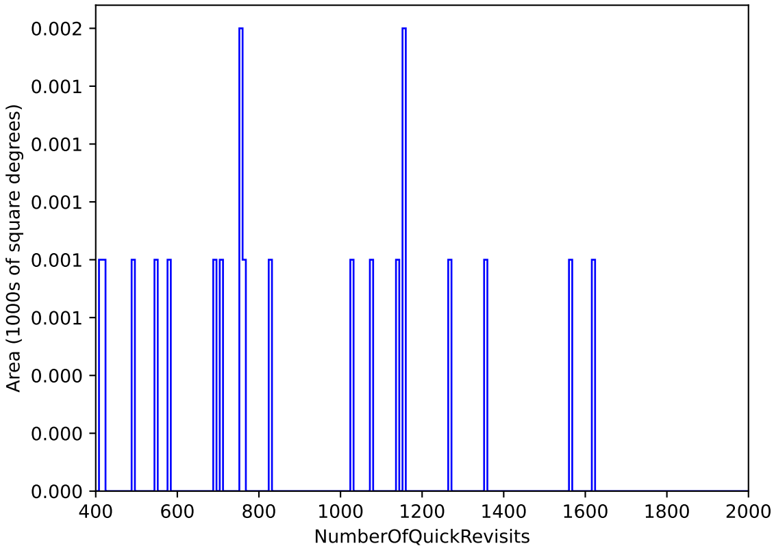
internal_u_expt45_nscale0.9v3.4_10yrs WFD: NumberOfQuickRevisits
