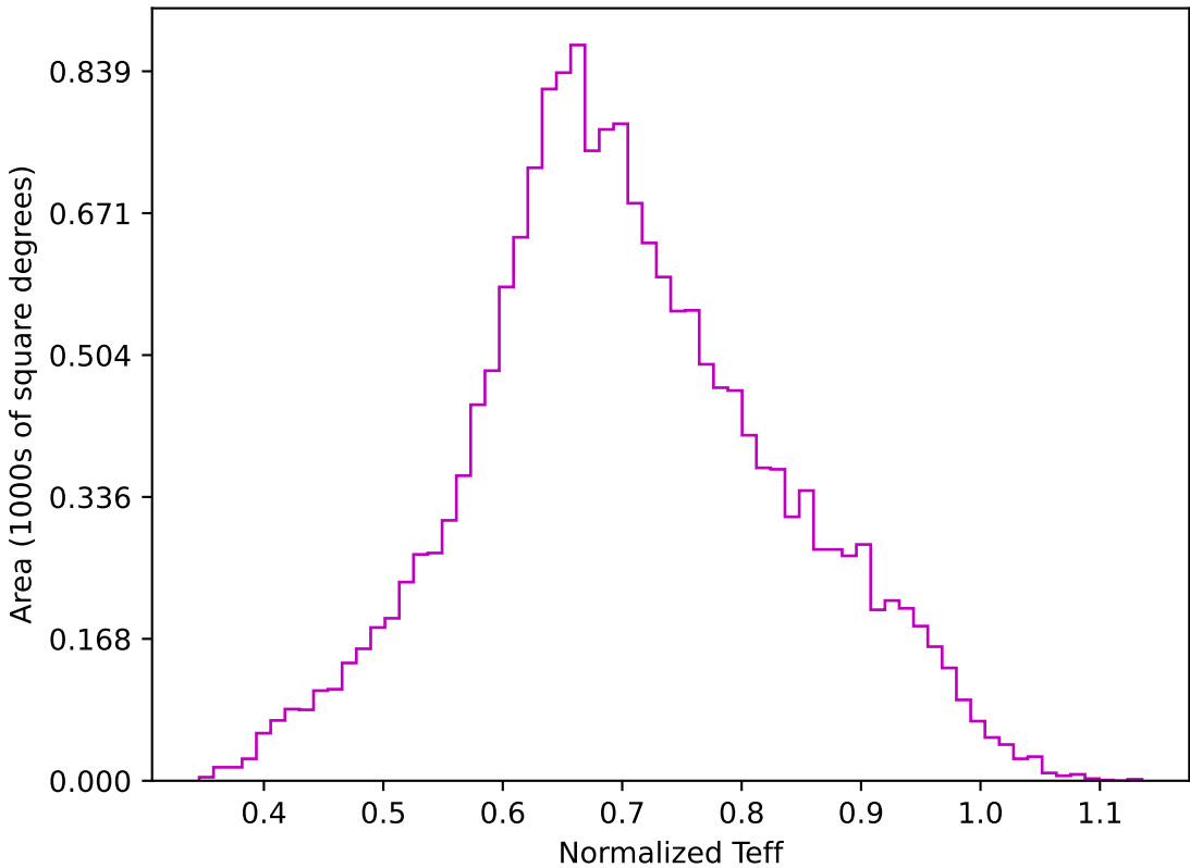
internal_u_expt45_nscale0.9v3.4_10yrs WFD z band: Normalized Teff
