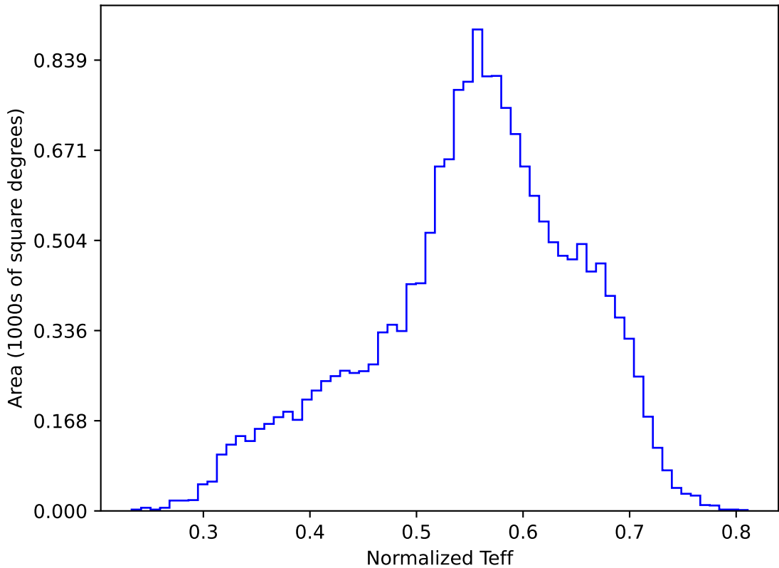
internal_u_expt45_nscale0.9v3.4_10yrs WFD y band: Normalized Teff
