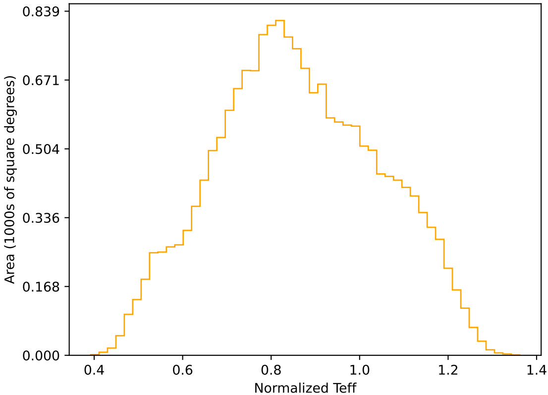
internal_u_expt45_nscale0.9v3.4_10yrs WFD r band: Normalized Teff
