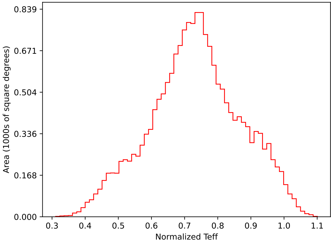
internal_u_expt45_nscale0.9v3.4_10yrs WFD i band: Normalized Teff
