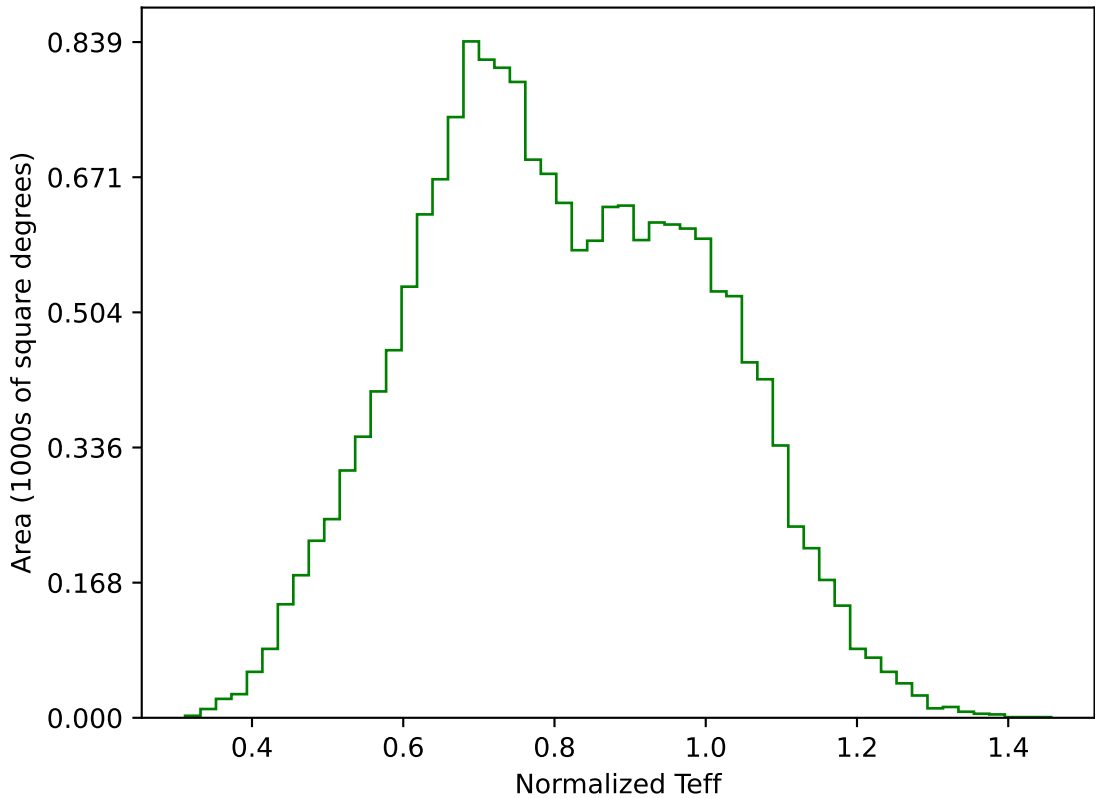
internal_u_expt45_nscale0.9v3.4_10yrs WFD g band: Normalized Teff
