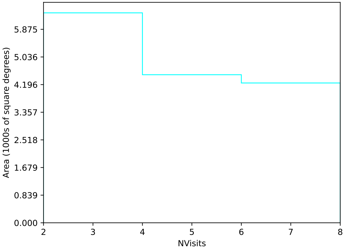
internal_u_expt45_nscale0.9v3.4_10yrs Yr 3-4 u band: NVisits
