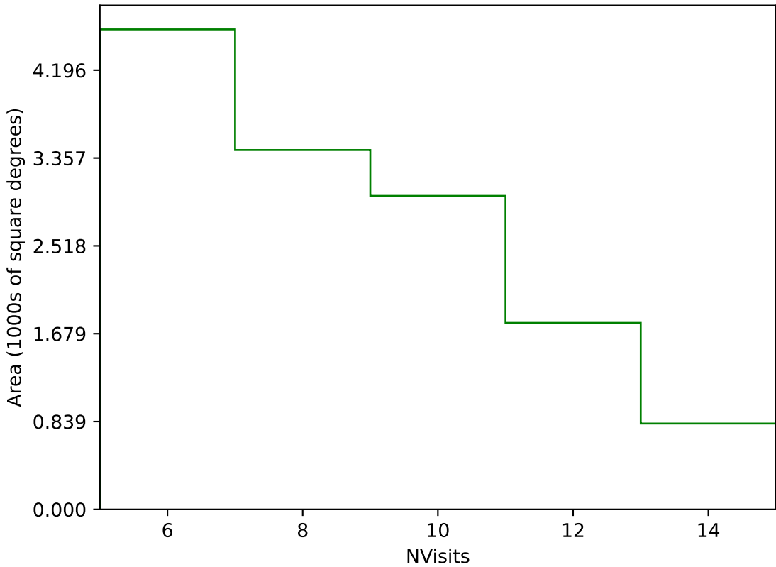
internal_u_expt45_nscale0.9v3.4_10yrs Yr 3-4 g band: NVisits
