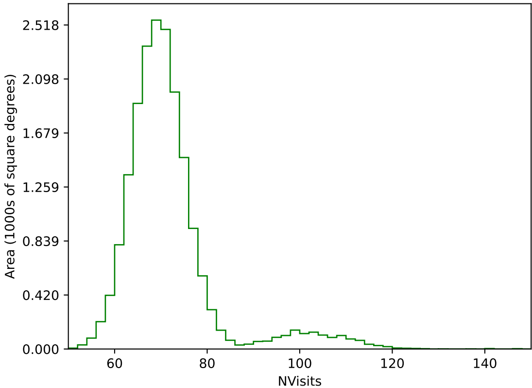
internal_u_expt45_nscale0.9v3.4_10yrs WFD g band: NVisits
