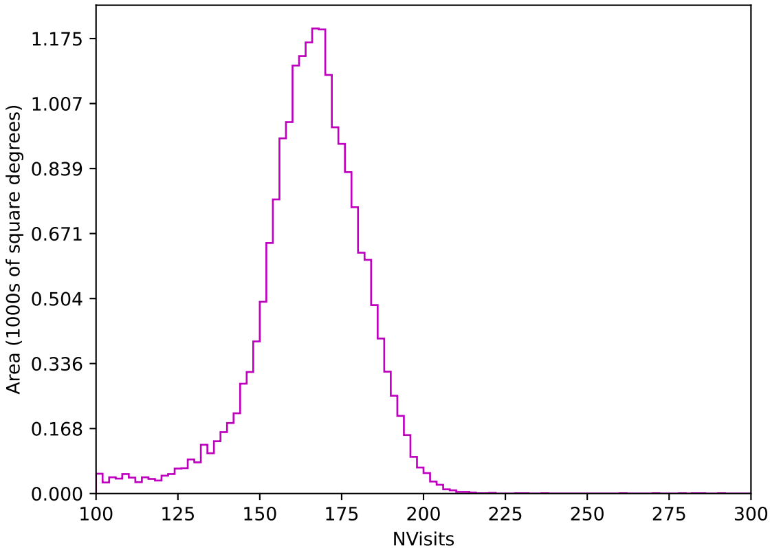
internal_u_expt45_nscale0.9v3.4_10yrs All sky z band: NVisits
