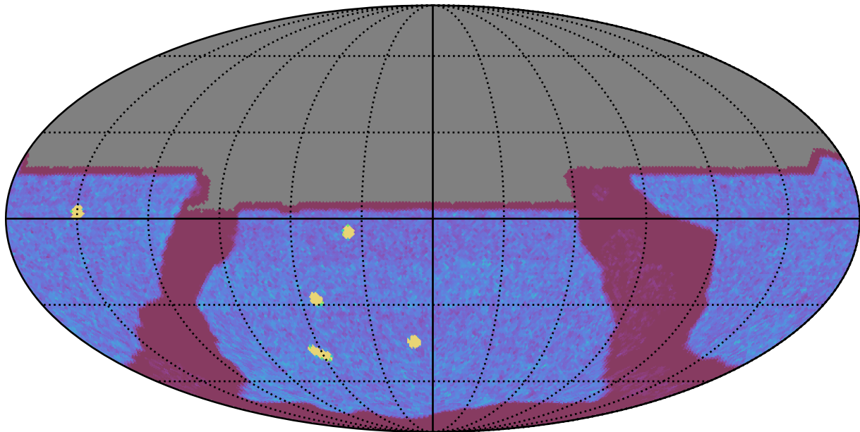
internal_u_expt45_nscale0.9v3.4_10yrs All sky y band: NVisits
