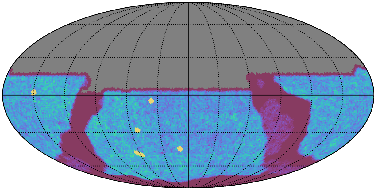
internal_u_expt45_nscale0.9v3.4_10yrs All sky u band: NVisits
