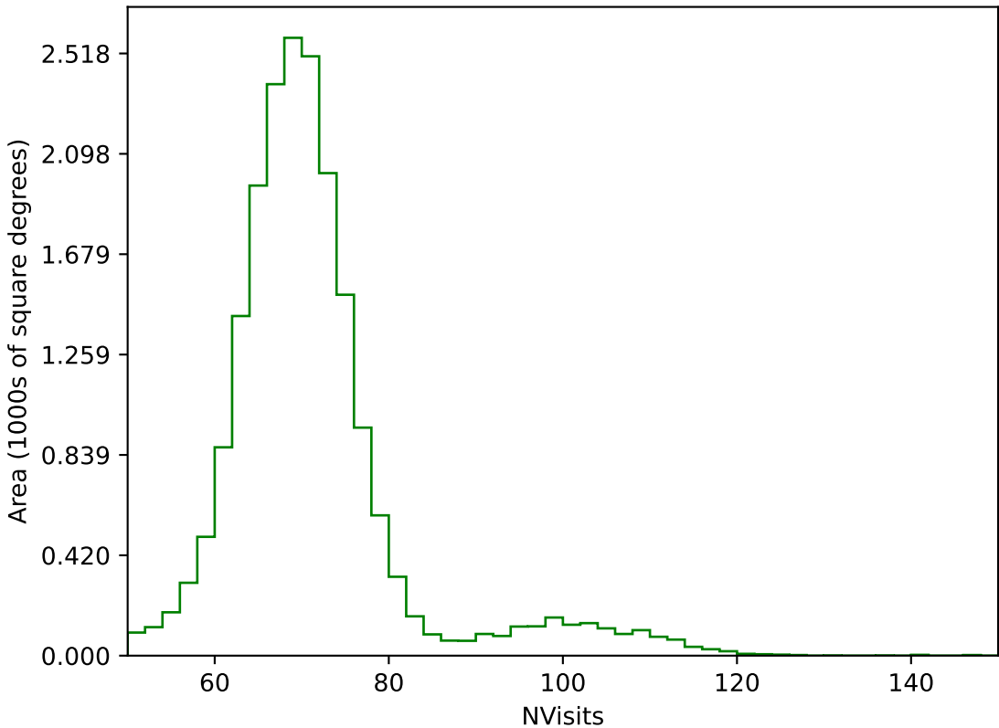
internal_u_expt45_nscale0.9v3.4_10yrs All sky g band: NVisits
