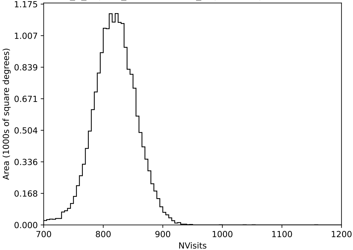
internal_u_expt45_nscale0.9v3.4_10yrs All sky all bands: NVisits
