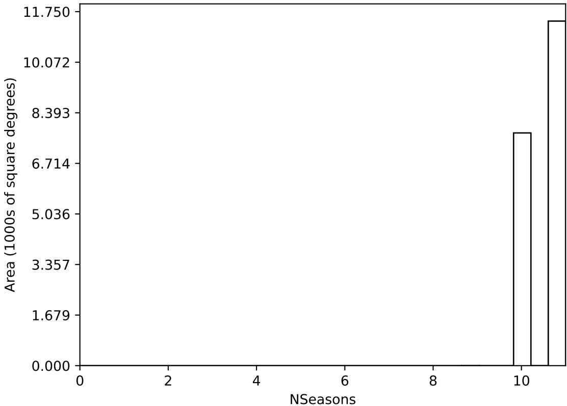
internal_u_expt45_nscale0.9v3.4_10yrs WFD all bands: NSeasons
