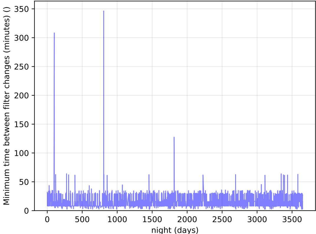
internal_u_expt45_nscale0.9v3.4_10yrs Per Night: Minimum time between filter changes (minutes)
