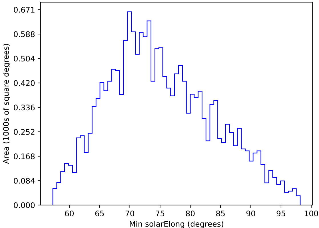
internal_u_expt45_nscale0.9v3.4_10yrs WFD g band: Min solarElong
