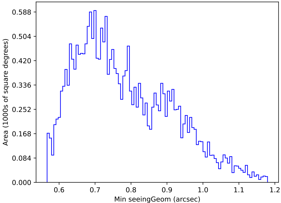
internal_u_expt45_nscale0.9v3.4_10yrs Yr 1 u band: Min seeingGeom
