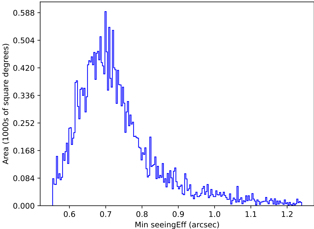
internal_u_expt45_nscale0.9v3.4_10yrs Yr 1 z band: Min seeingEff
