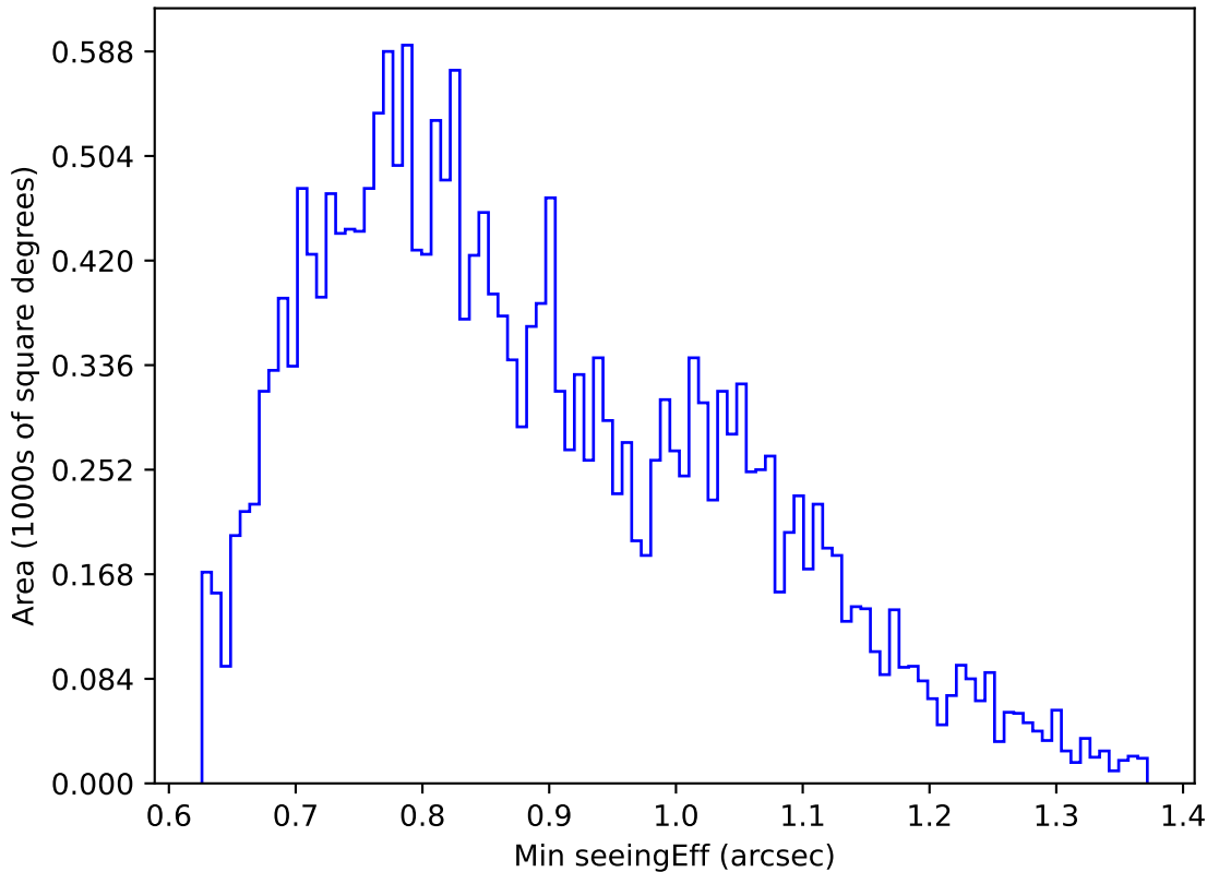
internal_u_expt45_nscale0.9v3.4_10yrs Yr 1 u band: Min seeingEff
