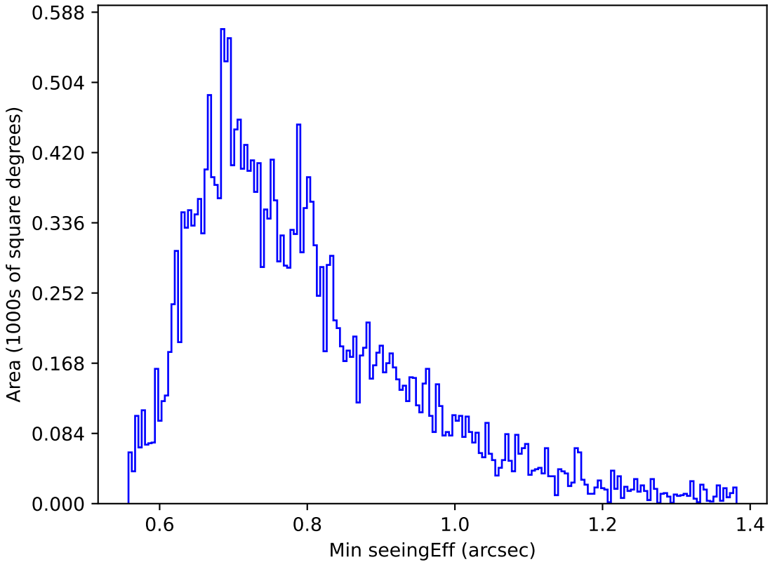
internal_u_expt45_nscale0.9v3.4_10yrs Yr 1 g band: Min seeingEff
