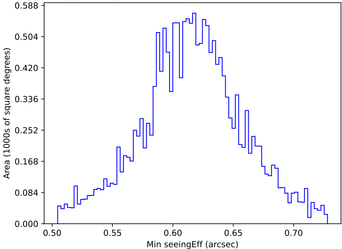
internal_u_expt45_nscale0.9v3.4_10yrs WFD z band: Min seeingEff
