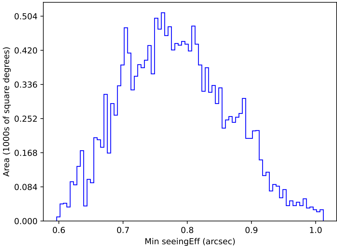
internal_u_expt45_nscale0.9v3.4_10yrs WFD u band: Min seeingEff
