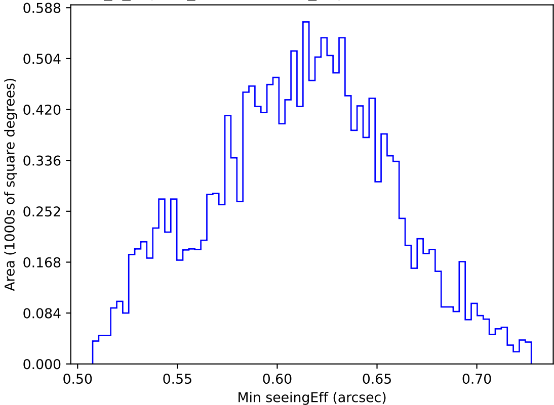
internal_u_expt45_nscale0.9v3.4_10yrs WFD r band: Min seeingEff
