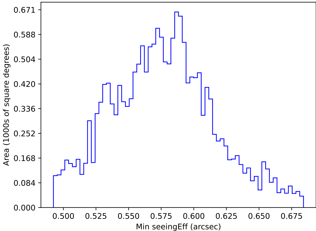
internal_u_expt45_nscale0.9v3.4_10yrs WFD all bands: Min seeingEff
