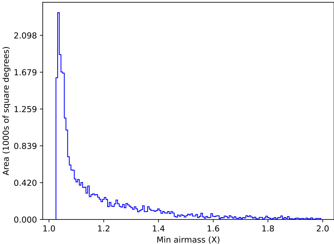
internal_u_expt45_nscale0.9v3.4_10yrs Yr 1 z band: Min airmass
