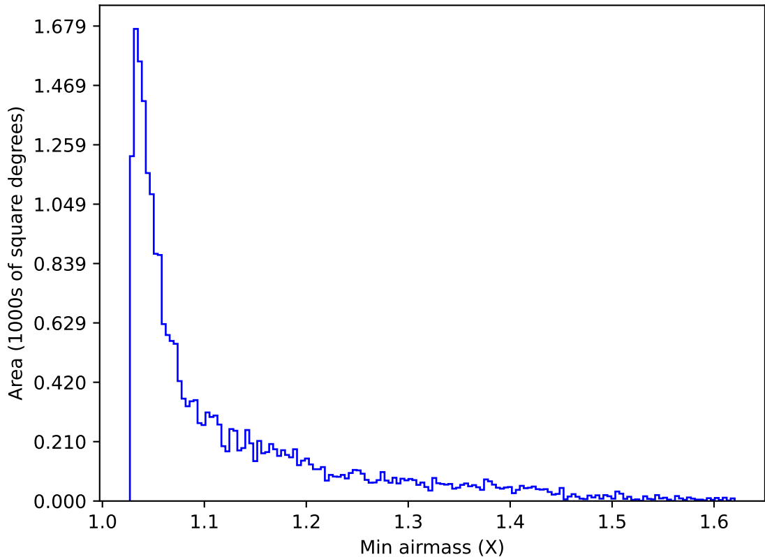
internal_u_expt45_nscale0.9v3.4_10yrs Yr 1 y band: Min airmass
