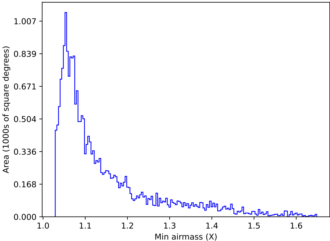
internal_u_expt45_nscale0.9v3.4_10yrs Yr 1 u band: Min airmass
