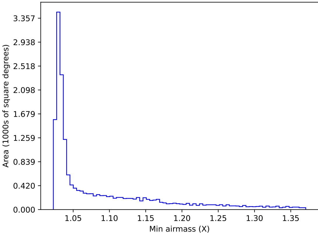
internal_u_expt45_nscale0.9v3.4_10yrs WFD y band: Min airmass
