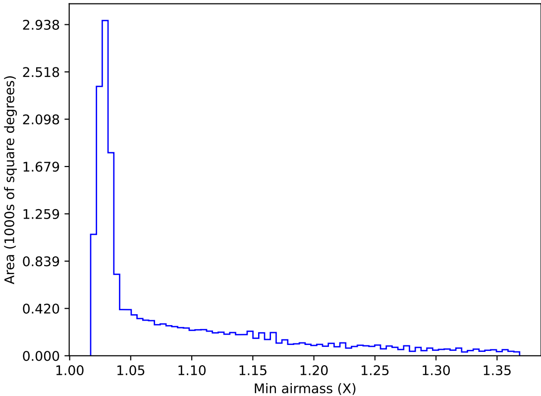
internal_u_expt45_nscale0.9v3.4_10yrs WFD r band: Min airmass
