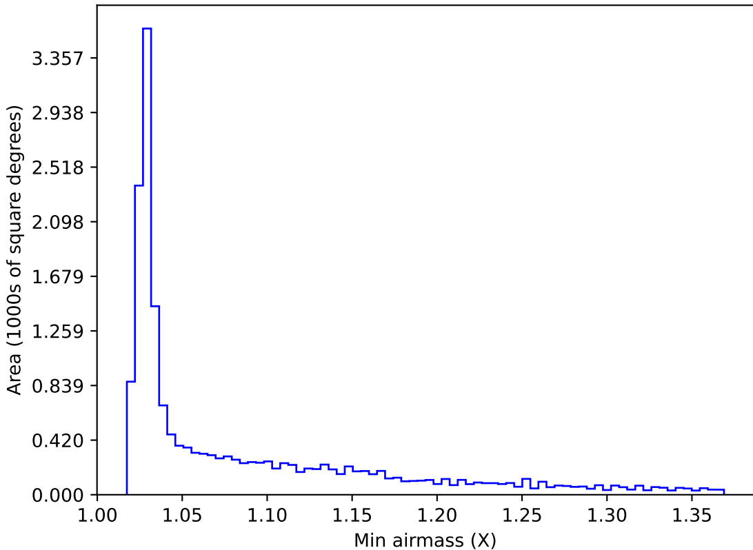
internal_u_expt45_nscale0.9v3.4_10yrs WFD i band: Min airmass
