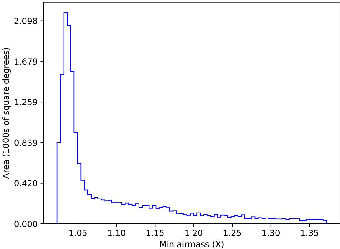
internal_u_expt45_nscale0.9v3.4_10yrs WFD g band: Min airmass
