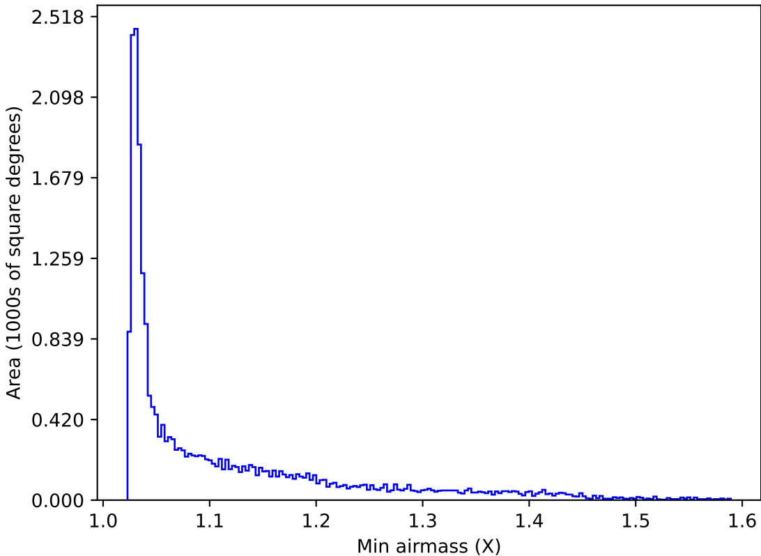
internal_u_expt45_nscale0.9v3.4_10yrs All sky y band: Min airmass
