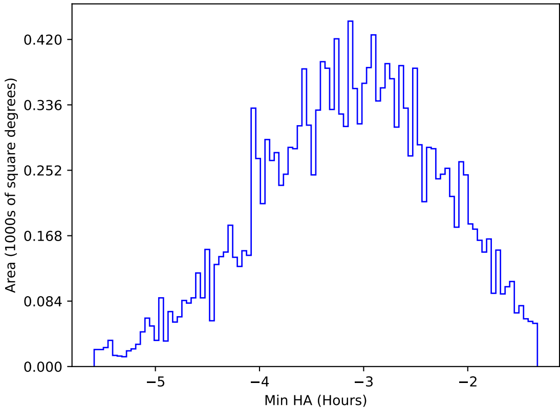
internal_u_expt45_nscale0.9v3.4_10yrs WFD u band: Min HA
