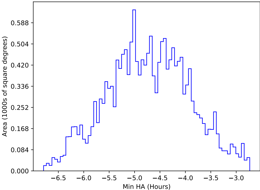
internal_u_expt45_nscale0.9v3.4_10yrs WFD all bands: Min HA
