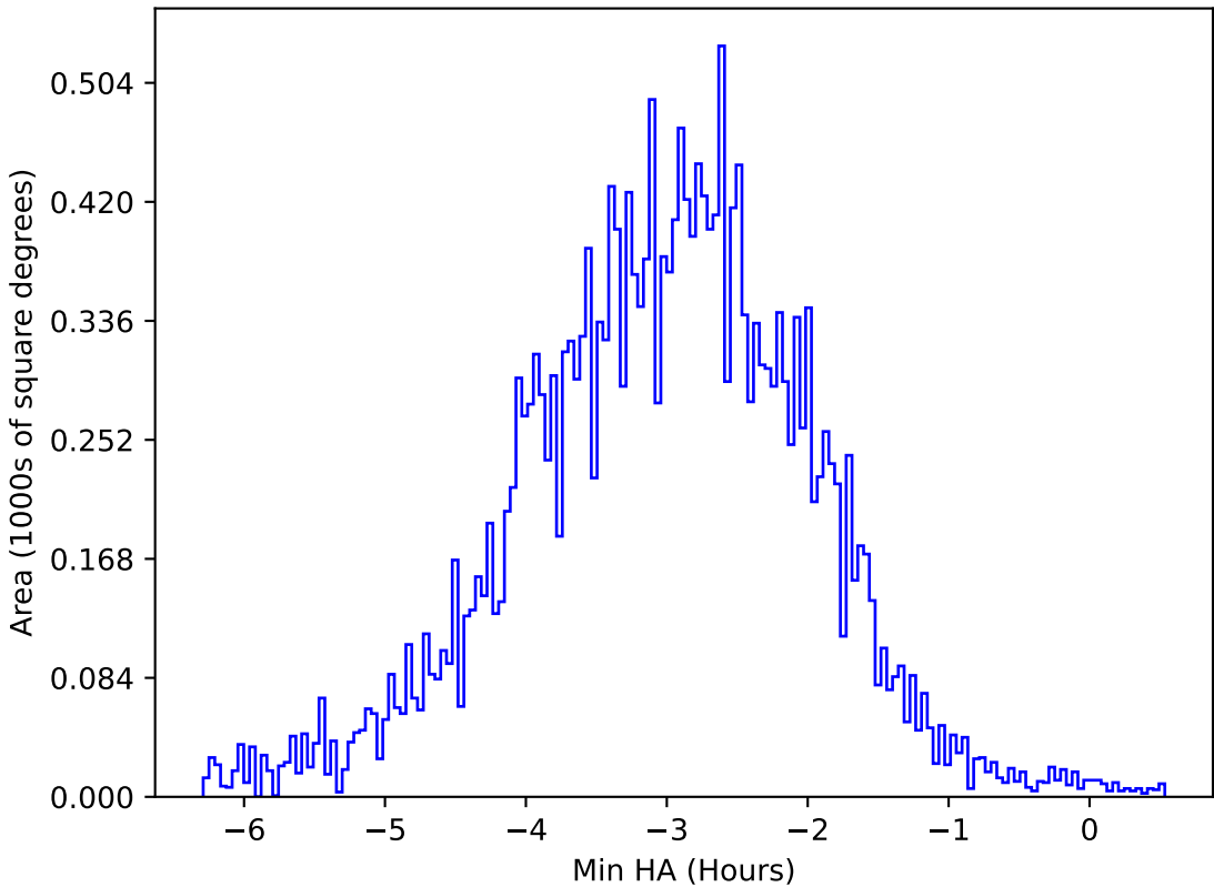
internal_u_expt45_nscale0.9v3.4_10yrs All sky u band: Min HA
