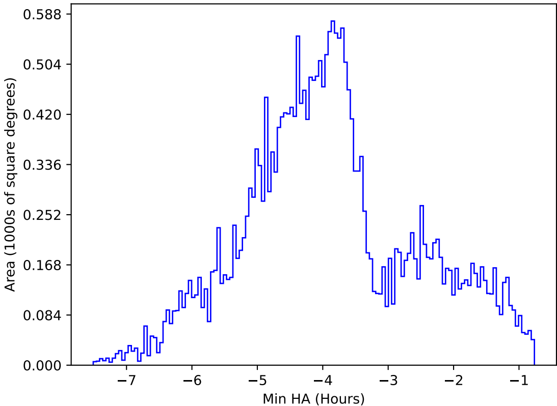
internal_u_expt45_nscale0.9v3.4_10yrs All sky g band: Min HA
