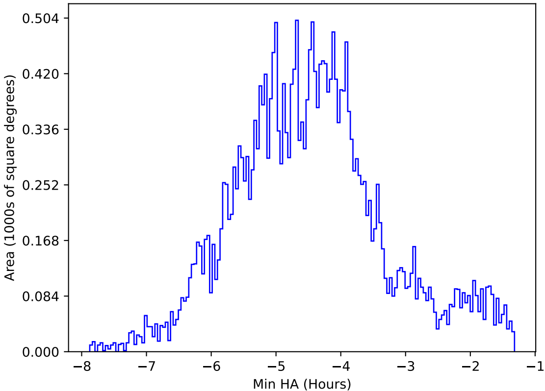
internal_u_expt45_nscale0.9v3.4_10yrs All sky all bands: Min HA
