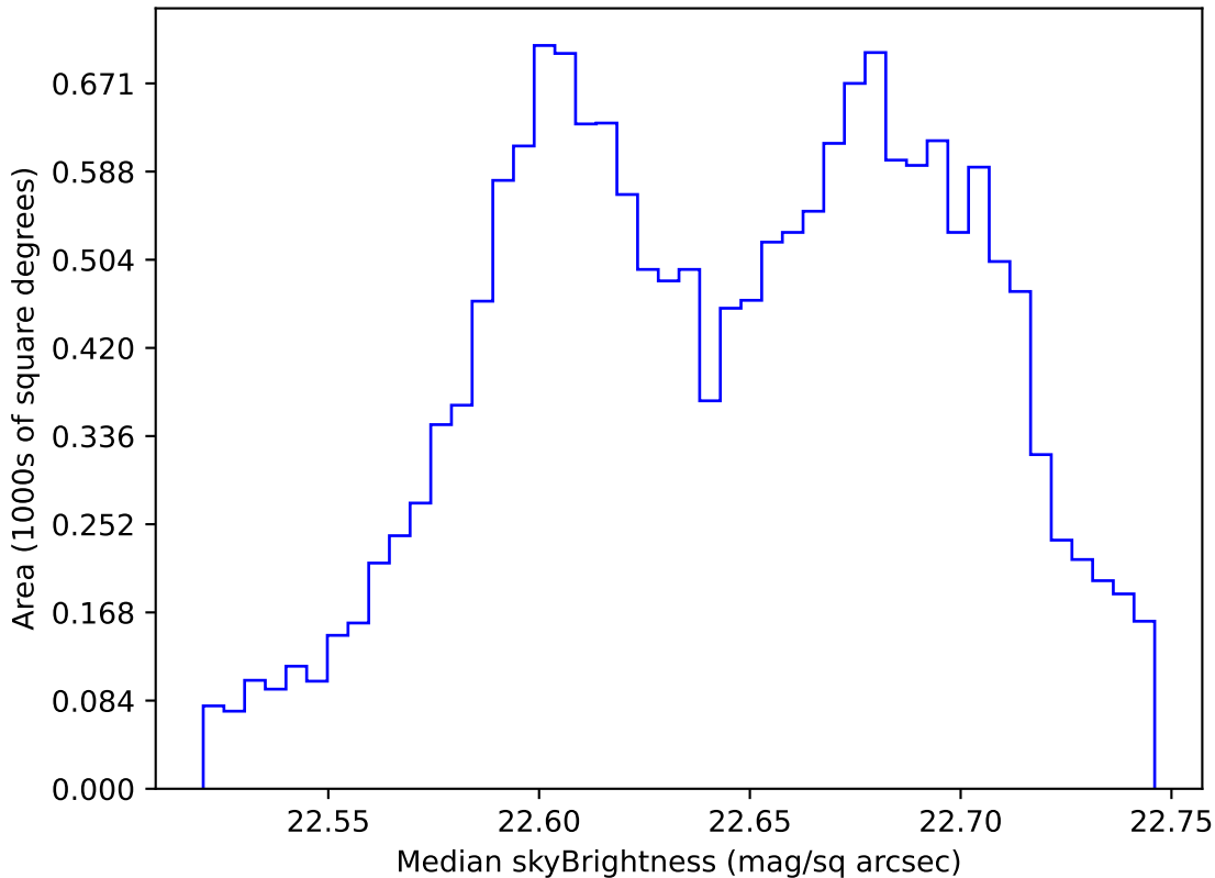
internal_u_expt45_nscale0.9v3.4_10yrs WFD u band: Median skyBrightness
