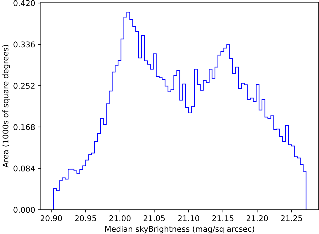
internal_u_expt45_nscale0.9v3.4_10yrs WFD r band: Median skyBrightness
