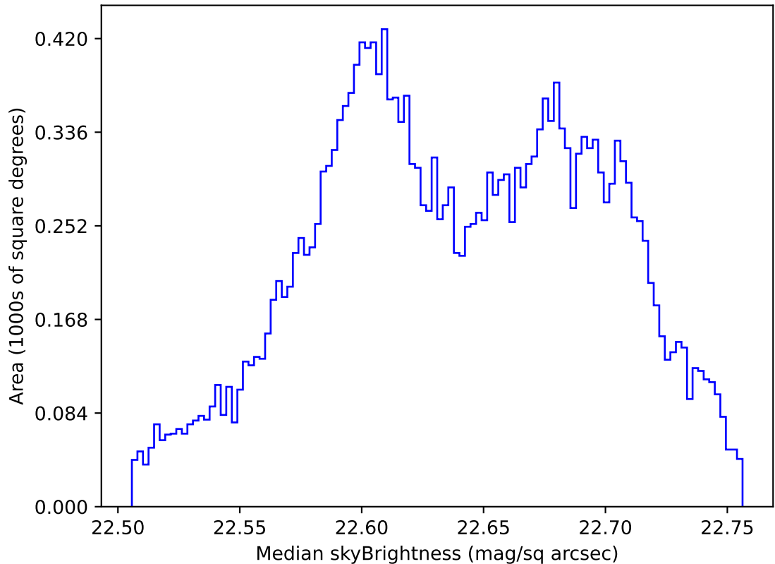
internal_u_expt45_nscale0.9v3.4_10yrs All sky u band: Median skyBrightness
