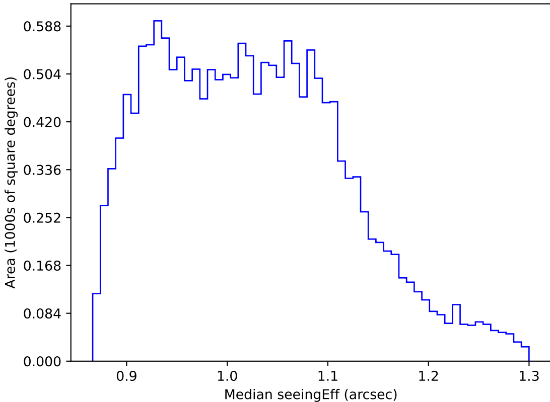
internal_u_expt45_nscale0.9v3.4_10yrs WFD r band: Median seeingEff
