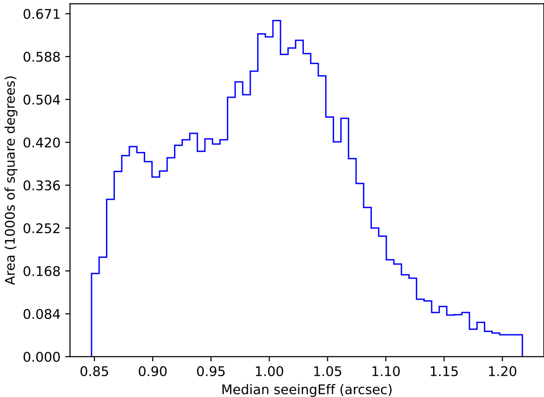
internal_u_expt45_nscale0.9v3.4_10yrs WFD i band: Median seeingEff
