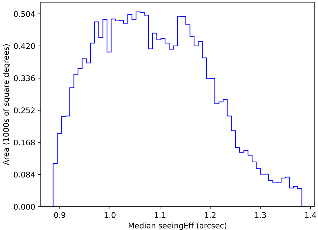
internal_u_expt45_nscale0.9v3.4_10yrs WFD g band: Median seeingEff
