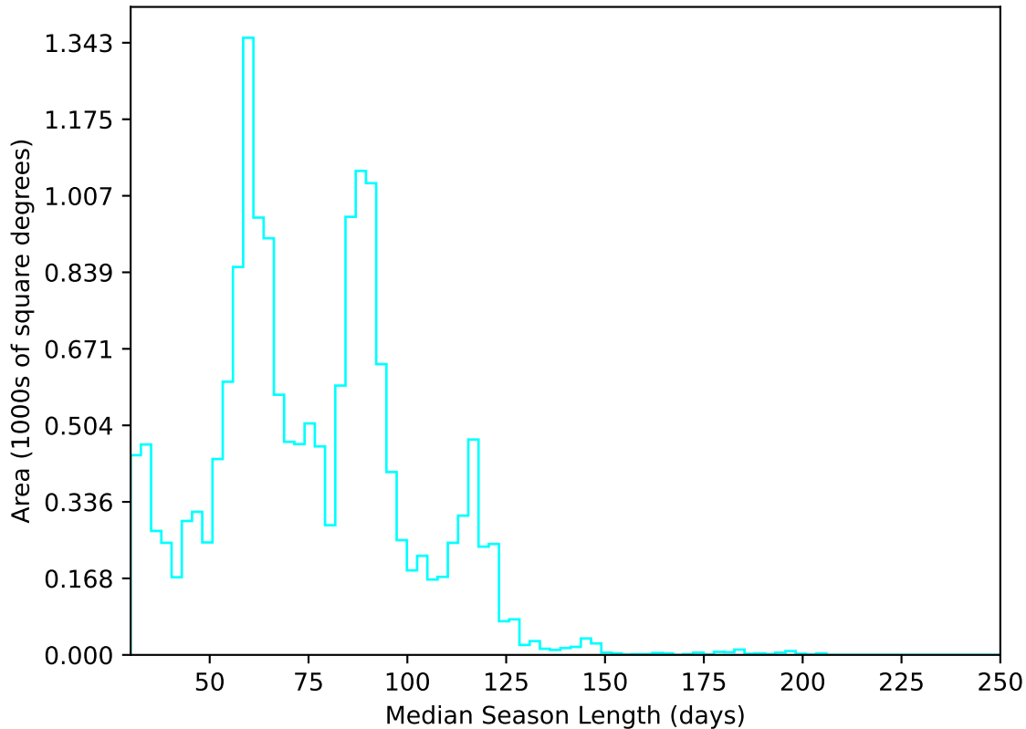
internal_u_expt45_nscale0.9v3.4_10yrs WFD u band: Median Season Length
