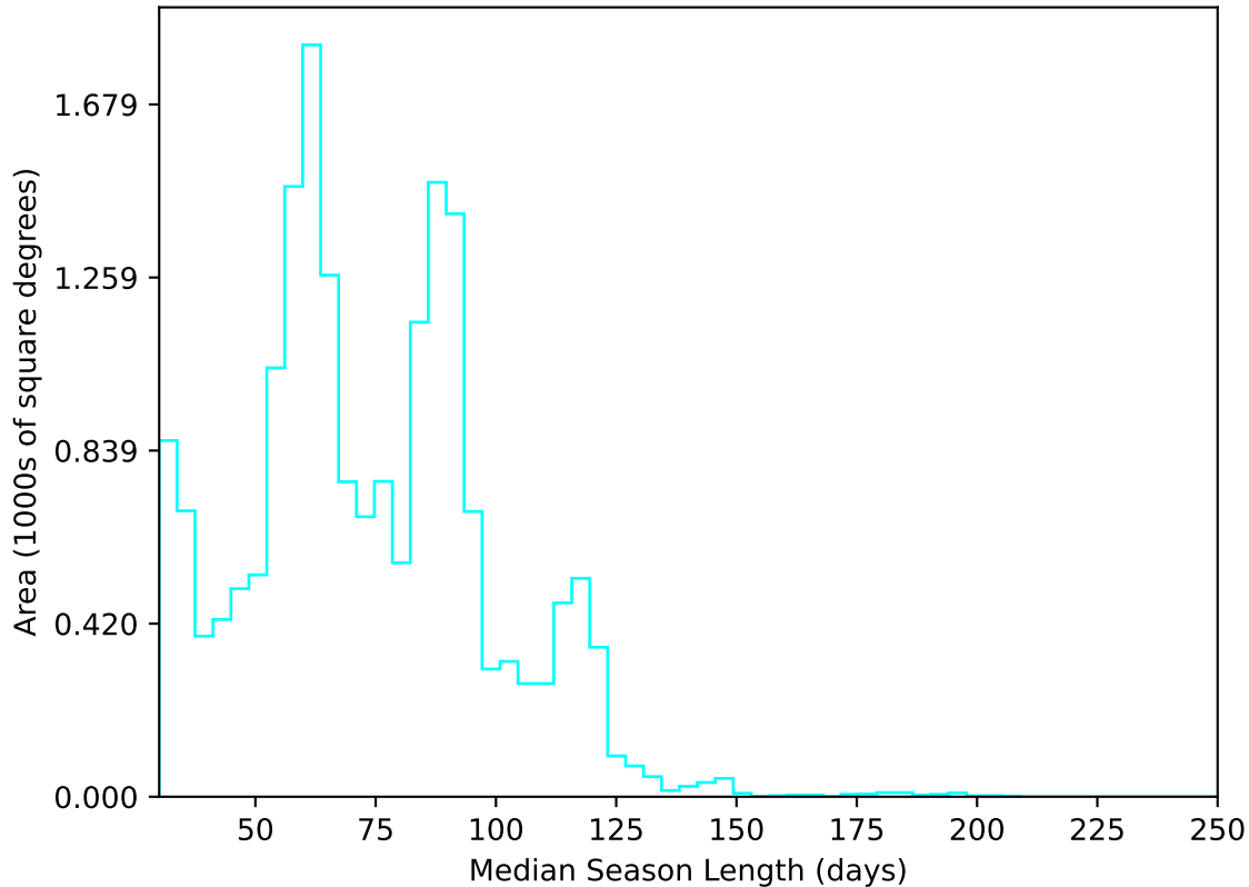
internal_u_expt45_nscale0.9v3.4_10yrs All sky u band: Median Season Length
