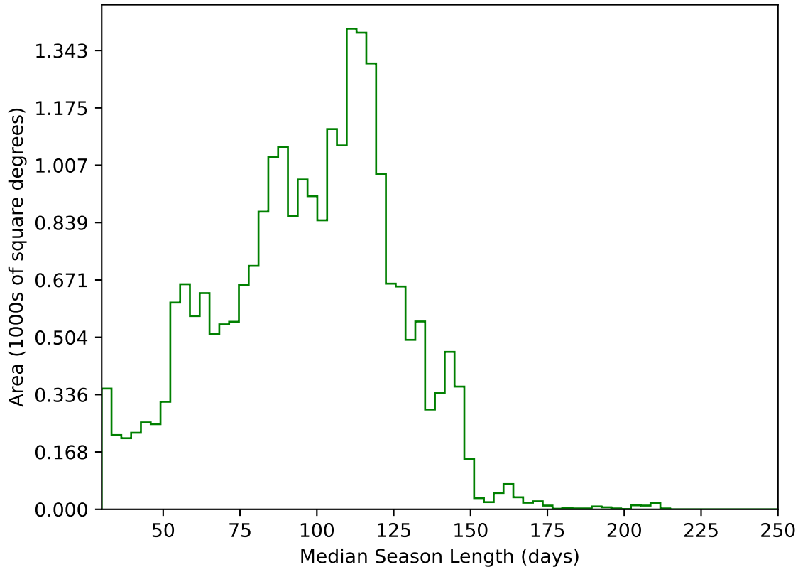
internal_u_expt45_nscale0.9v3.4_10yrs All sky g band: Median Season Length
