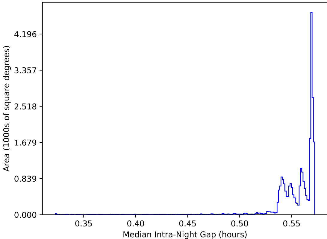
internal_u_expt45_nscale0.9v3.4_10yrs All sky: Median Intra-Night Gap
