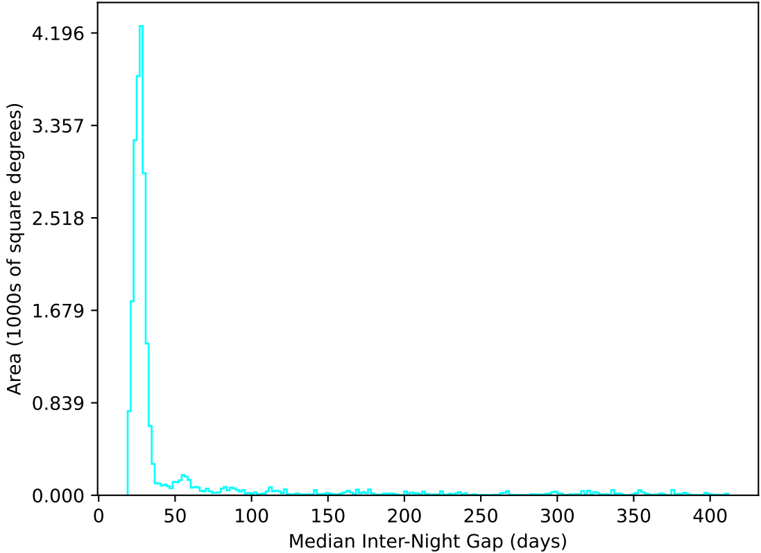
internal_u_expt45_nscale0.9v3.4_10yrs All sky u band: Median Inter-Night Gap
